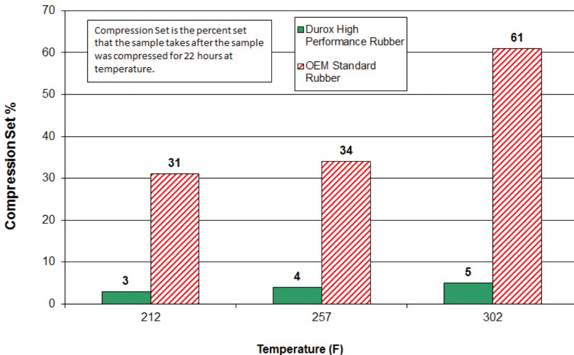
Durox - Seal Test Compression Set Test @ 22 Hours
